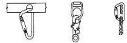
CORRECT CONNECTIONS
